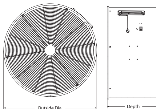
Figure 1 — Dimensions
